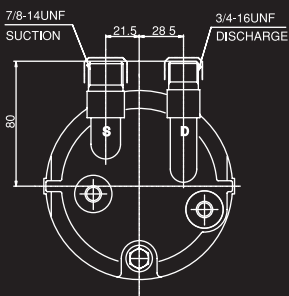
O-RING TYPE MOUNTING
