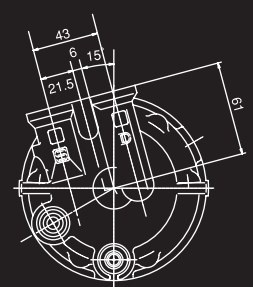
VERTICAL PAD TYPE
